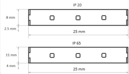
cutting section and dimensions
